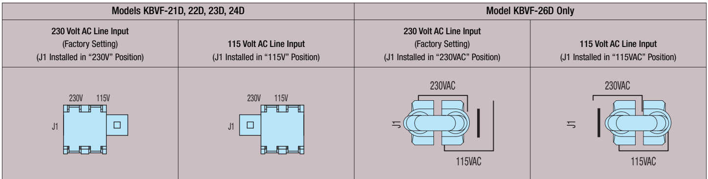
FIGURE 10 - AC LINE INPUT VOLTAGE SELECTION (DUAL VOLTAGE MODELS ONLY) (J1 is located on the Upper PC Board)
