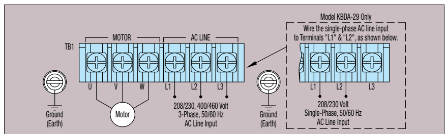
FIGURE 8 – MODELS KBDA-29 1 , 45 2 , 48 2 MOTOR, AC LINE INPUT & GROUND CONNECTIONS
