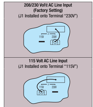
FIGURE 6 – MODELS KBDA-24D*, 27D AC LINE INPUT VOLTAGE SELECTION
