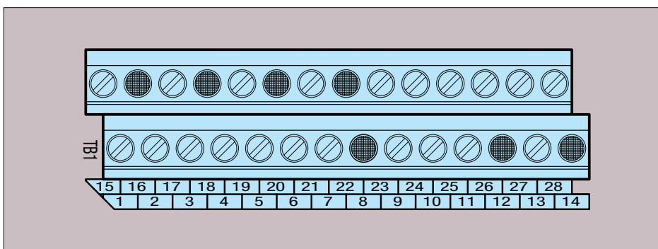
FIGURE 2 – IODA TERMINAL BLOCK TB1 LAYOUT
