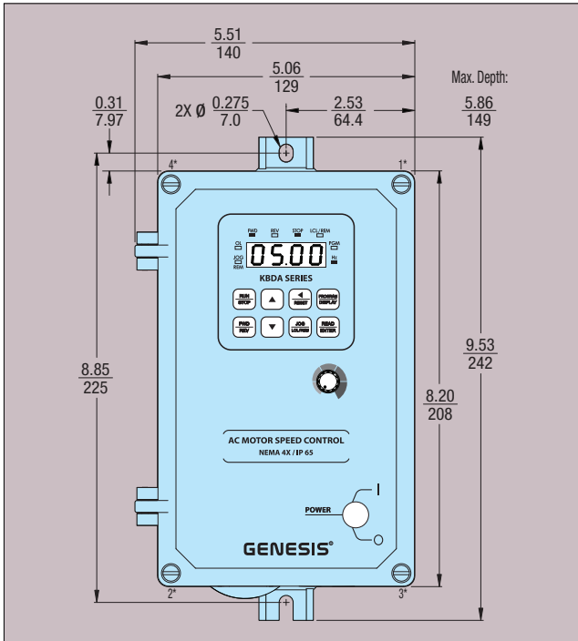
FIGURE 3 – MODEL KBDA-24D MECHANICAL SPECIFICATIONS (Inches/mm)
