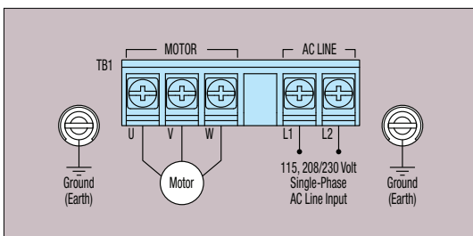
FIGURE 7 – MODELS KBDA-24D, 27D* MOTOR, AC LINE INPUT & GROUND CONNECTIONS
