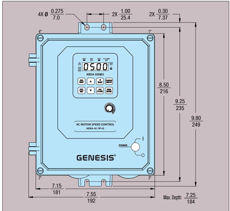
FIGURE 4 – MODELS KBDA-27D, 29, 45, 48 MECHANICAL SPECIFICATIONS (Inches/mm)
