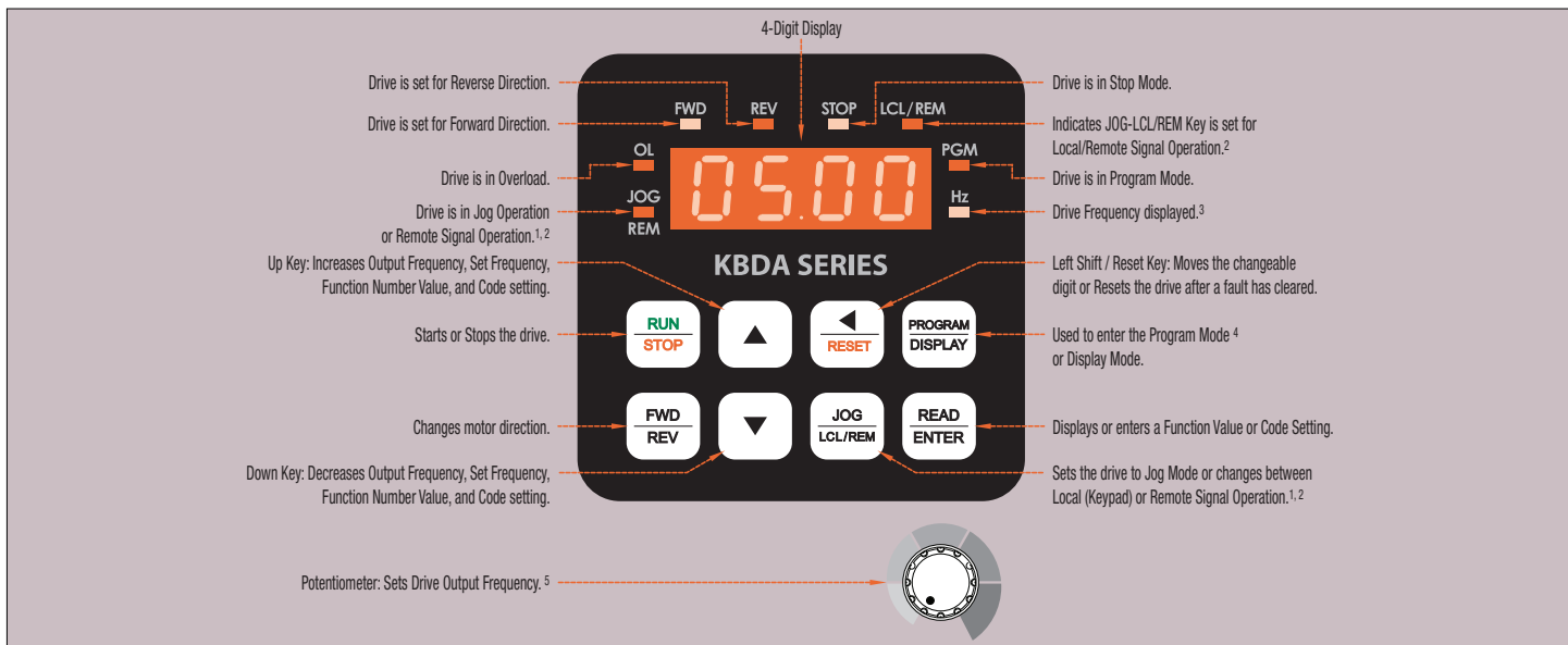
FIGURE 1 – KEYPAD LAYOUT
