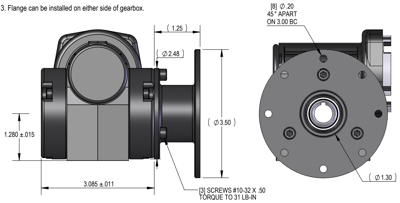
FLANGE INSTALLED ON 3F/H GEARBOX
