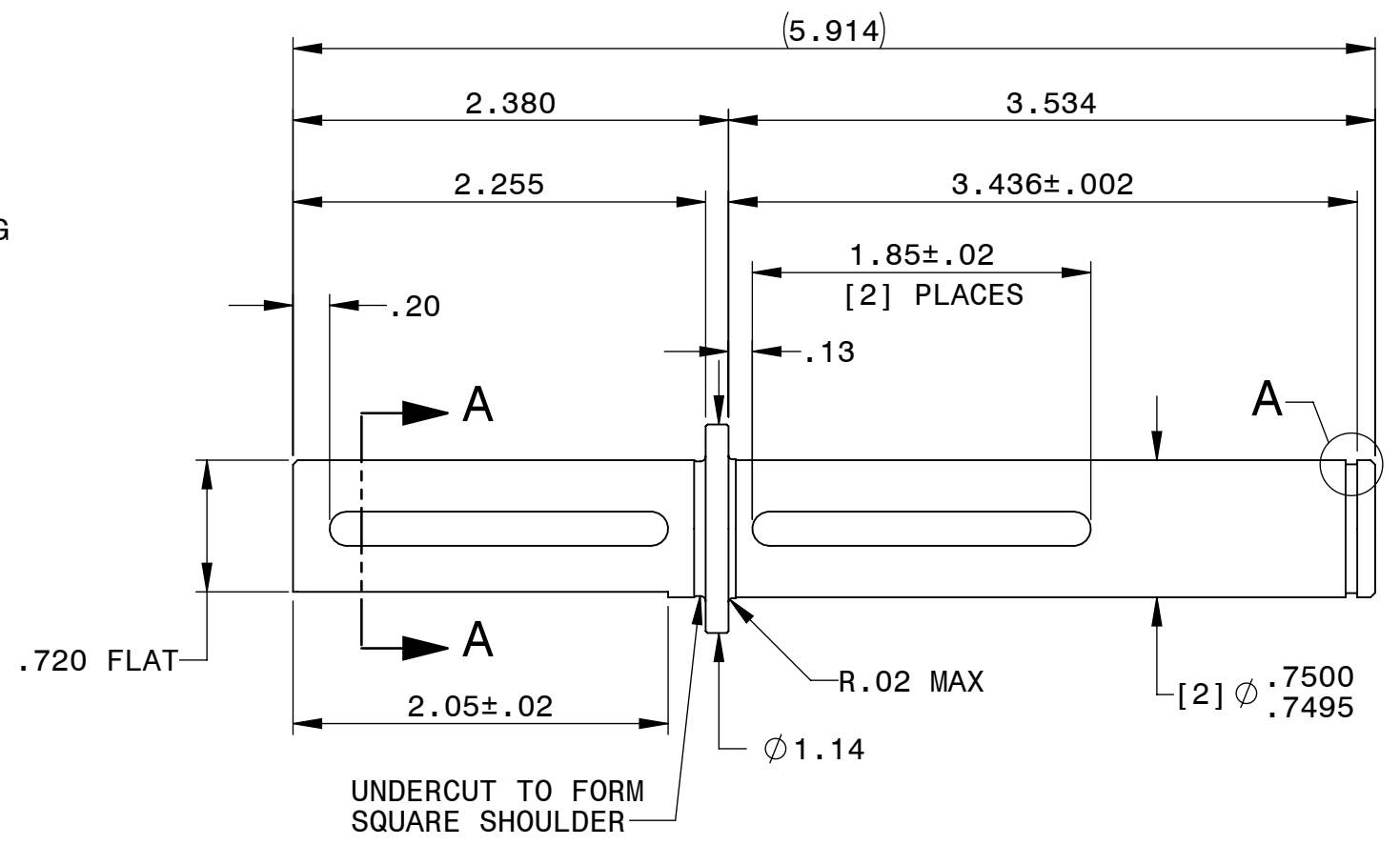
SHAFT DIMENSIONS
