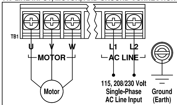
FIGURE 11 KBAC-24D, 27D*, 29 (1P) AC LINE INPUT, MOTOR, AND GROUND CONNECTIONS
