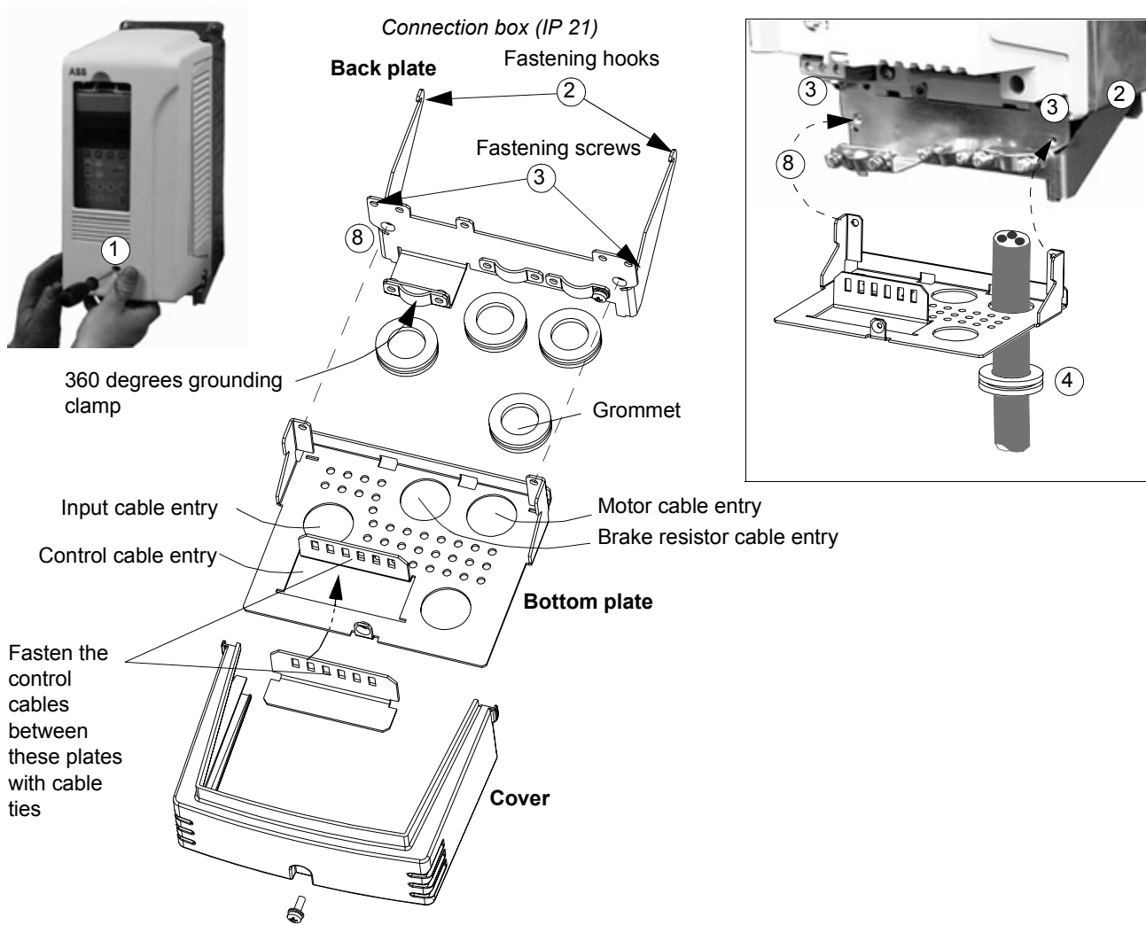
Frame sizes R2 to R4
