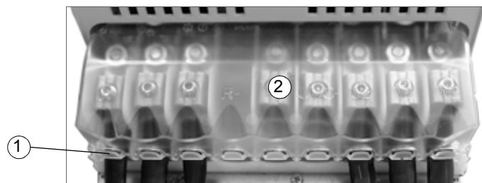
View of cable terminal installation
